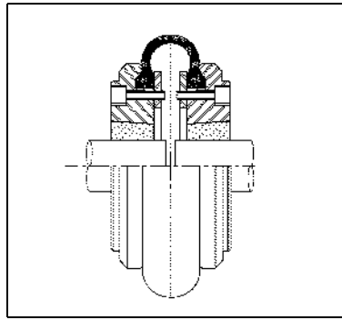
SIZES F40-60
