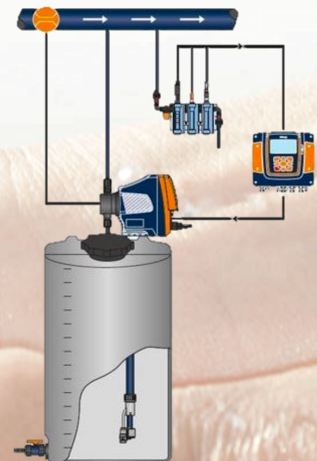
Motor-driven Metering pump
